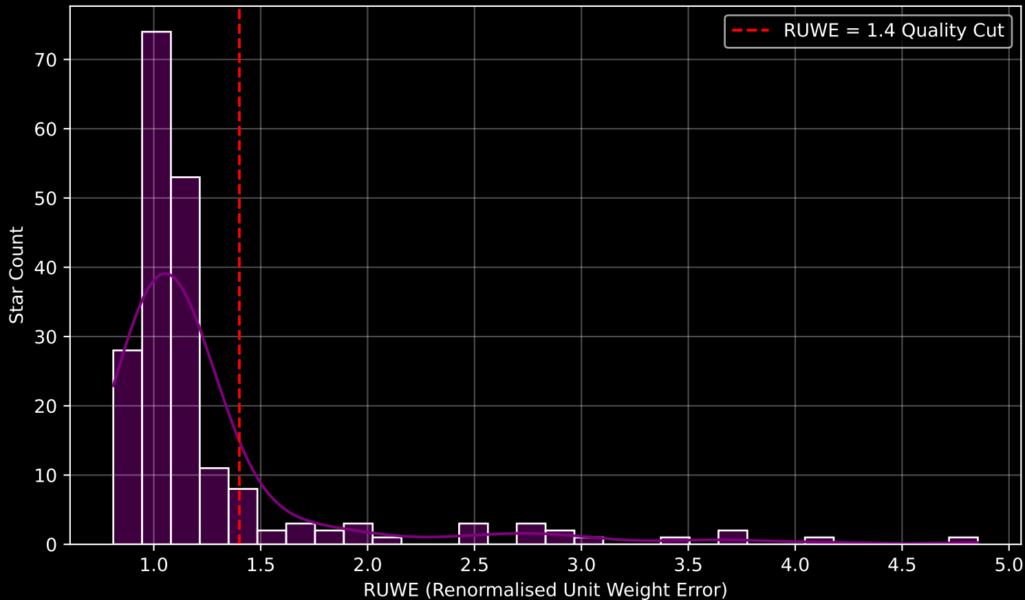
GAPOGEE DR17 Field [074-35_MGA] RUWE Distribution (n= 199)
