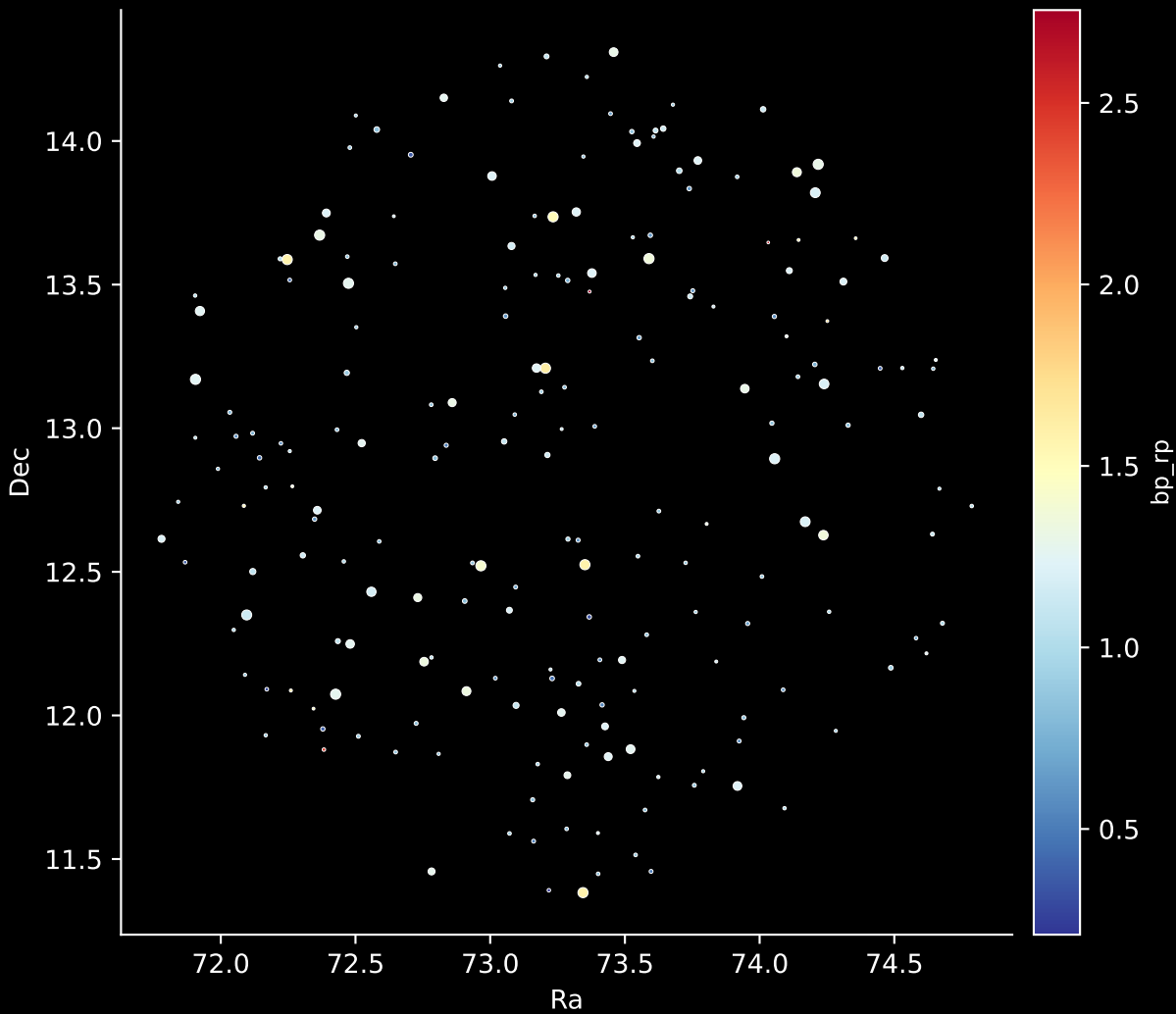
APOGEE DR17 Field: [074-35_MGA] Stars: 202
