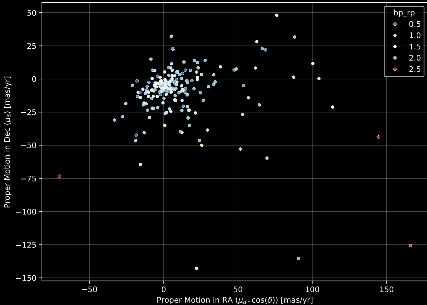
APOGEE DR17 Field: [074-35_MGA] Proper Motion Diagram (n= 202)
