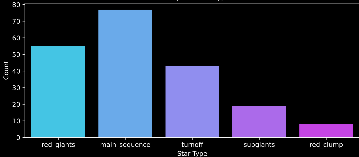
APOGEE DR17 Field: [074-35_MGA] Count plot of Star Type
