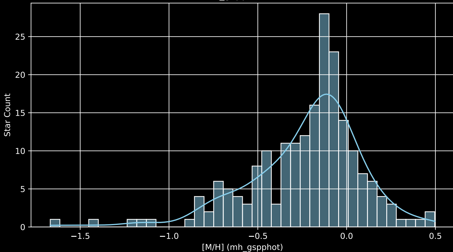
APOGEE DR17 Field: [074-35_MGA [M/H] (mh_gspphot) (n= 201)
