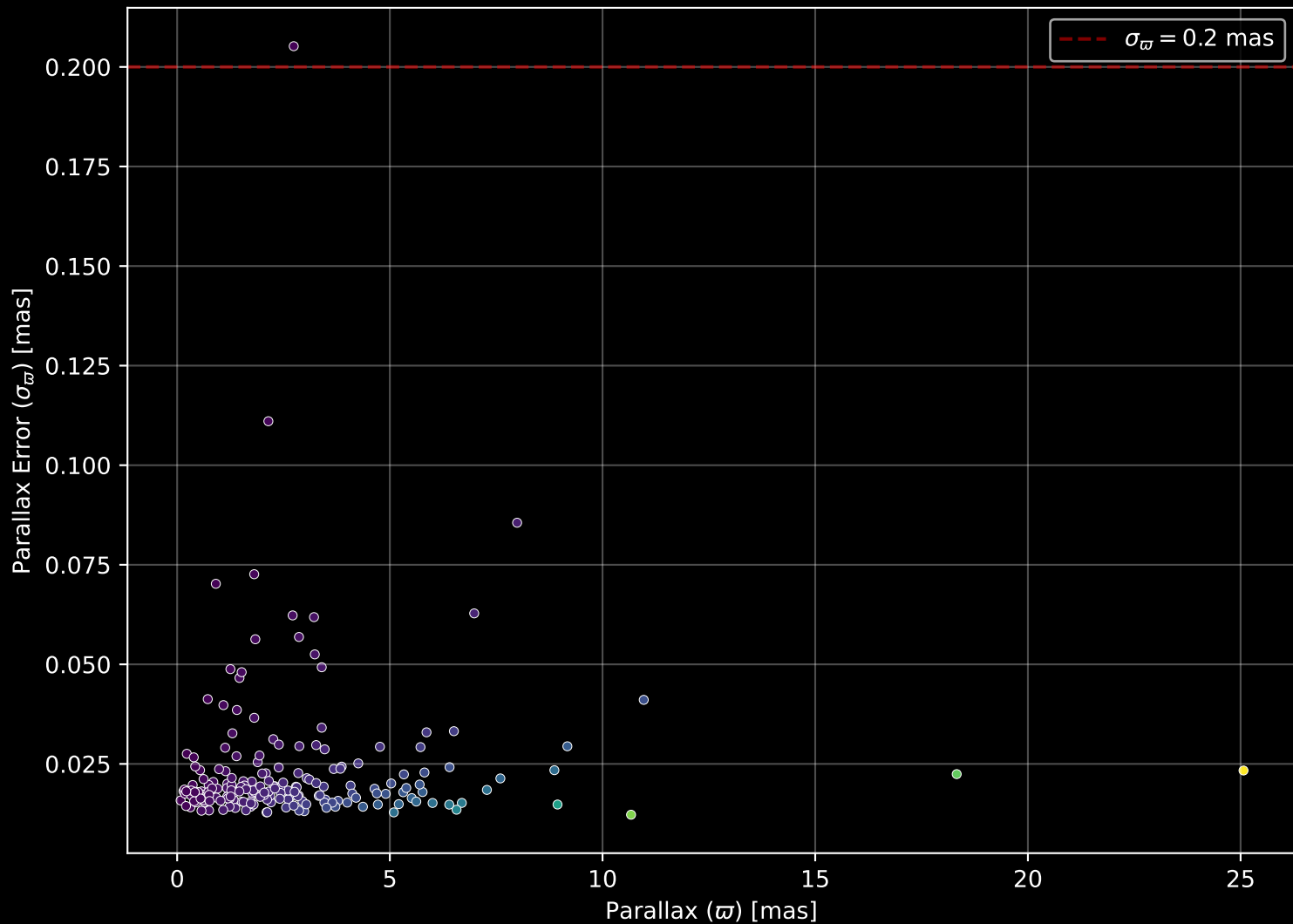
APOGEE DR17 Field: [074-35_MGA] Parallax Quality (n= 202)
